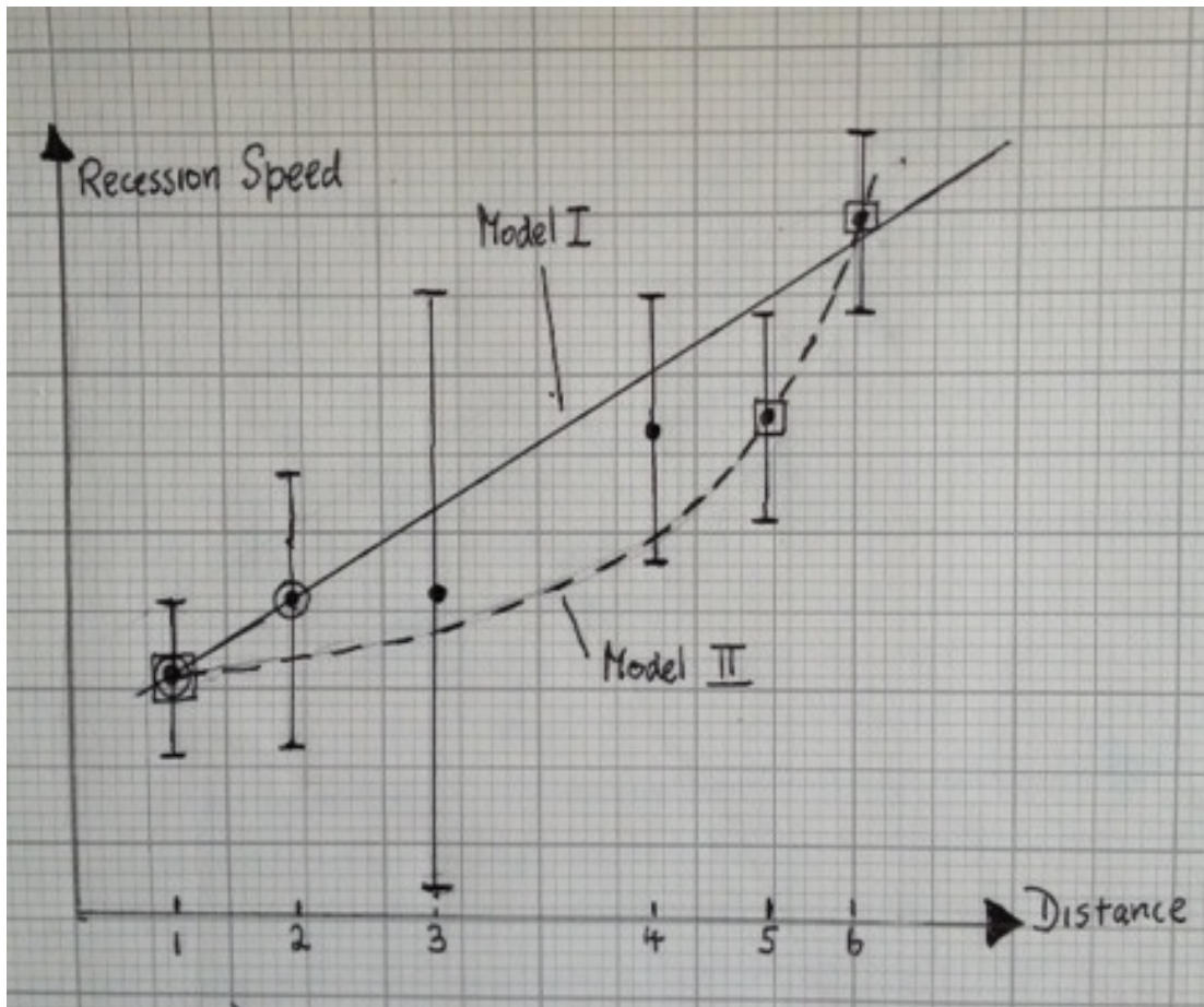
Fig 1: Astronomer X's recession speeds (with error bars) for 6 white nebulae labelled 1 to 6, plotted against rough estimates of their relative distances. No scales are shown or were needed to test his hypothesis of expansion. The Model I line is for steady expansion, the Model II curve is for slowing expansion due to gravity; it's steeper in the past, i.e. in the distance.
